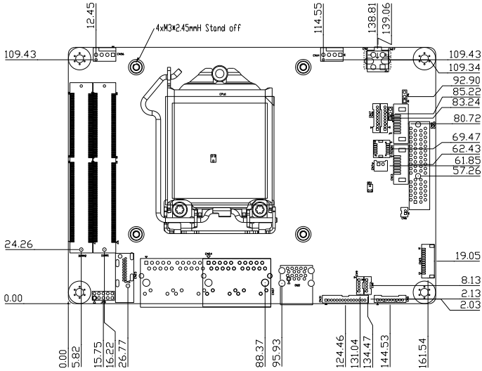
Component Side
