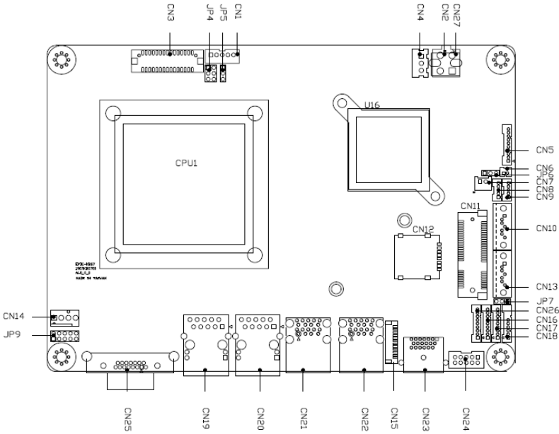
Component Side
