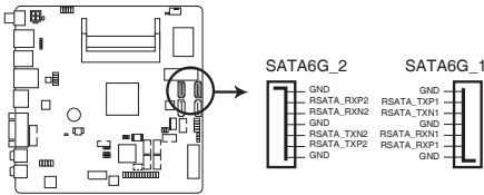
EMB-BT4 SATA 6.0Gb/s connectors
