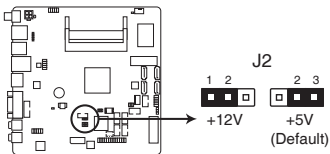
EMB-BT4 Inverter Voltage Selection
