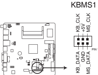
EMB-BT4 Series PS/2 keyboard/mouse connector
