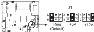
EMB-BT4 COM1 Ring/+5V/+12V Selection
