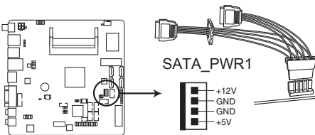
EMB-BT4 SATA POWER Connector
