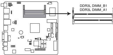
EMB-BT4 204-pin DDR3L DIMM sockets
