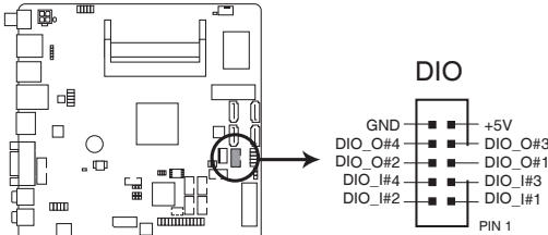
EMB-BT4 DIO connector
