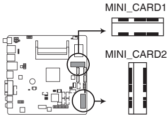
EMB-BT4 MINICARD connectors
