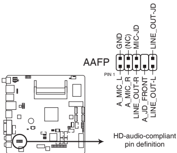
EMB-BT4 Front panel audio connector
