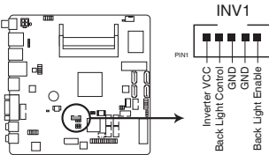
EMB-BT4 Inverter connector
