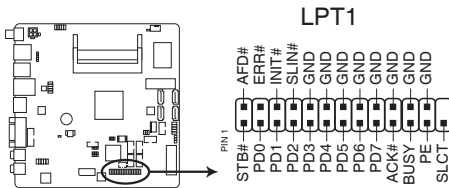
EMB-BT4 Parallel Port Connector
