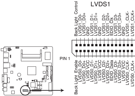
EMB-BT4 LVDS connector
