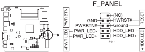
EMB-BT4 System panel connector
