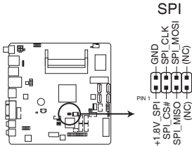
EMB-BT4 BIOS Programmable Connector
