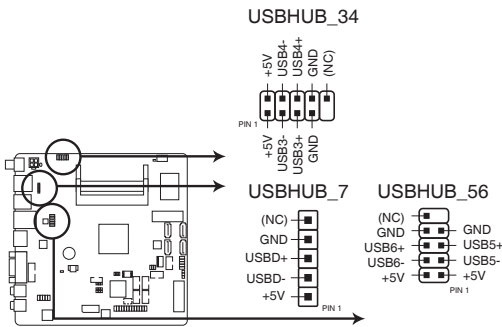
EMB-BT4 USB2.0 connectors
