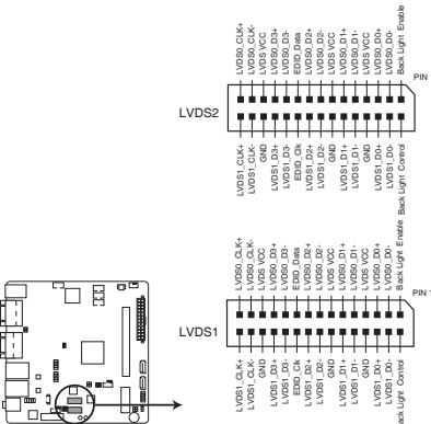
EMB-BT2 LVDS Panel Signal connectors
