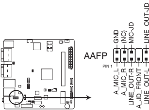
EMB-BT2 Front panel audio connector
