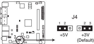
EMB-BT2 LVDS1 Panel Voltage selection
