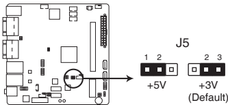
EMB-BT2 LVDS2 Panel Voltage selection
