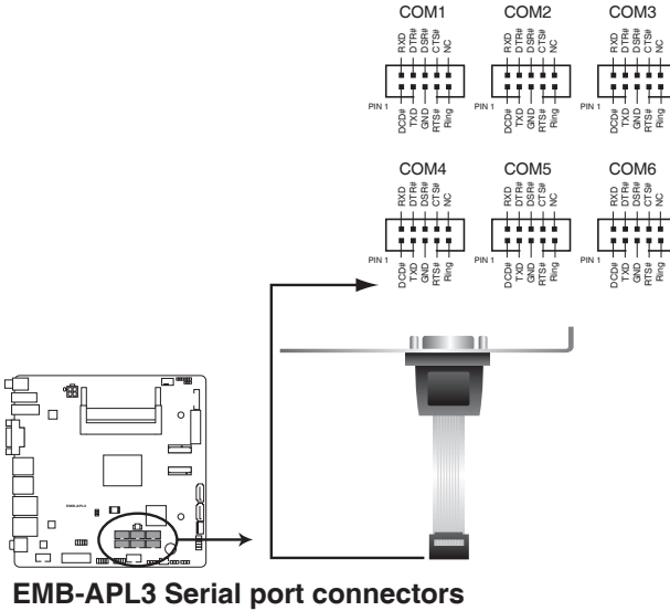
EMB-APL3 Serial port connectors
