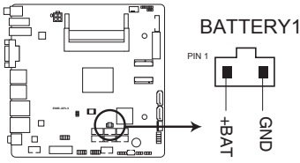
EMB-APL3 Battery connector
