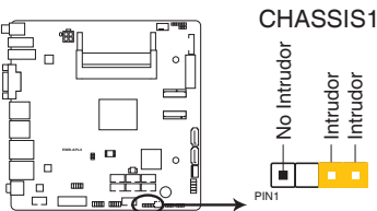
EMB-APL3 Chassis intrusion connector
