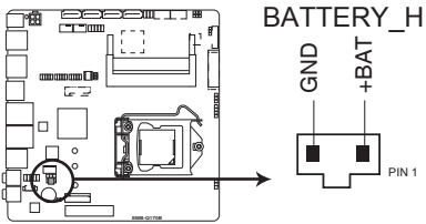
EMB-Q170B Battery Holder connector
