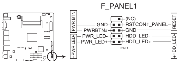
EMB-APL1 System panel connector
