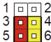
Pins 3-5 and 4-6 selected
