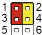
Pins 1-3 and 2-4 selected +5V_DUAL for ATX (Default)
