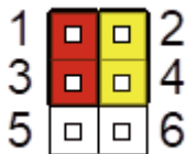
Pins 1-3 and 2-4 selected
