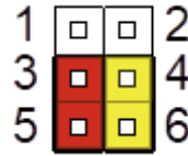
Pins 3-5 and 4-6 selected CAN Bus
