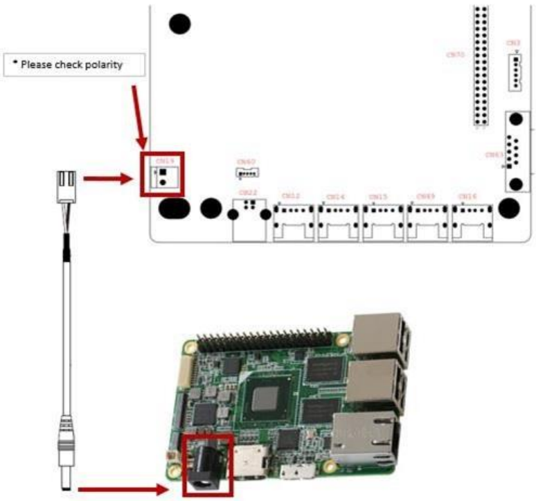
Wiring Diagram 4:
