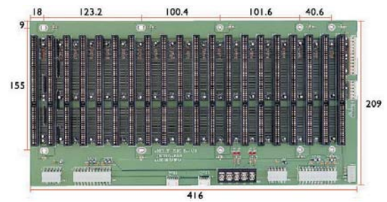
BP-220SI-V60 Single System, 20xISA
