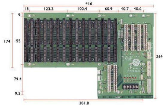
BP-219SG-P4-V60 4xPCI, 13xISA, 2xPICMG
