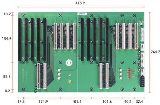
BP-218DG-P9-V61 8xPCI, 6xISA, 4xPICMG
