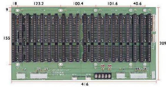
BP-220DI-V60 Dual System, 20xISA
