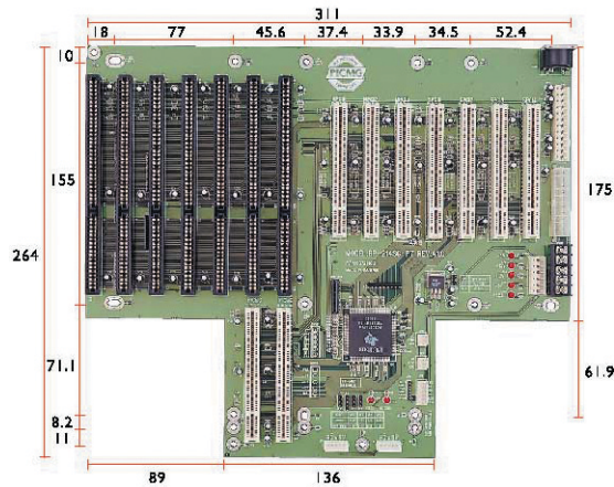
BP-214SG-P7-V22 7xPCI, 5xISA, 2xPICMG
