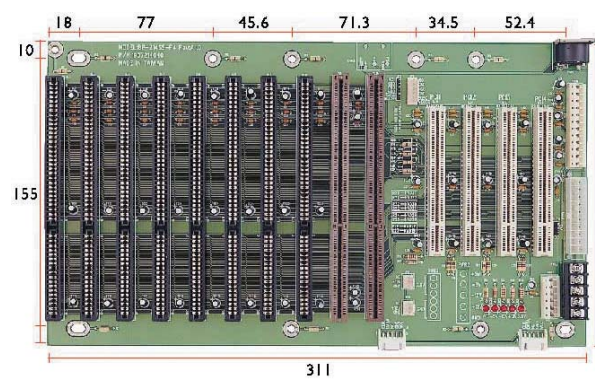
BP-214SS-P4-V11 4xPCI, 2xPCISA, 8xISA
