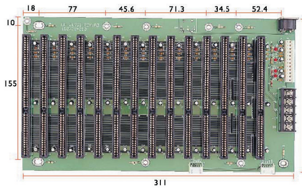
BP-214SI-V61 14xISA
