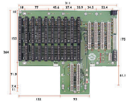
BP-214SG-P4-V65 4xPCI, 8xISA, 2xPICMG
