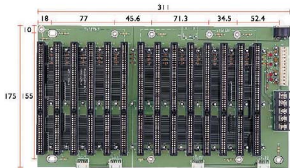
BP-214DI-V60 Dual System, 14xISA
