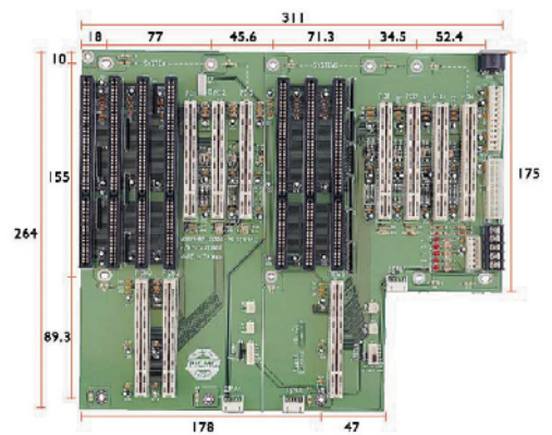
BP-213DG-P6-V60 Dual System, 7xPCI, 4xISA, 3xPICMG
