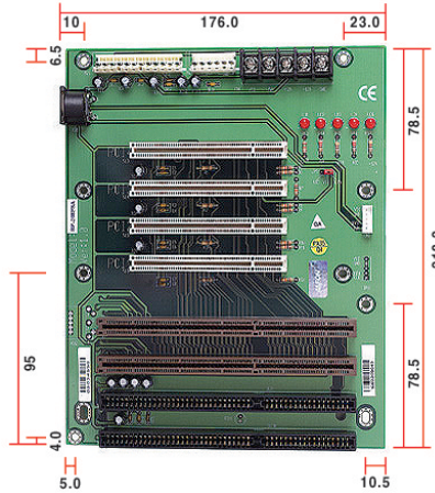
BP-208SS-P4-V10 2xPCI, 4xISA, 2xPCISA
