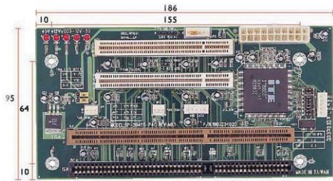
BP-204SS-P2-A10 1xPCI, 1xPCISA, 1xISA, 1xPCI (PICMG)
