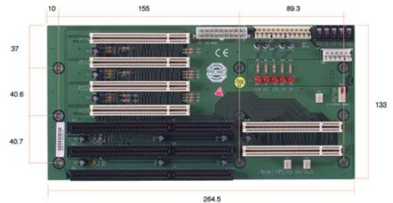
BP-206SG-P3-V61 4xPCI, 1xISA, 2xPICMG
