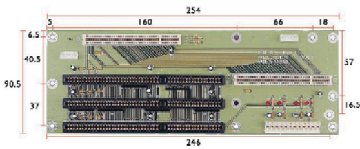
BP-204SG-P1-A10 1xPCI, 2xISA, 1xPICMG
