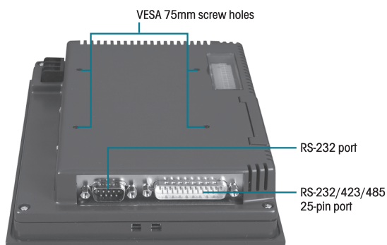
VESA 75mm screw holes
