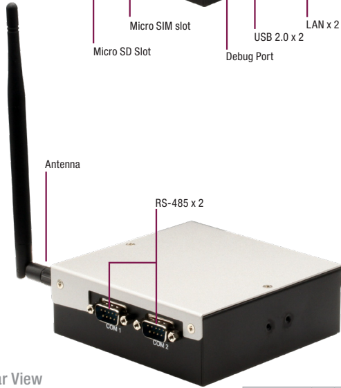
Rear View
