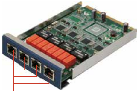
LAN, RJ-45 x 4
