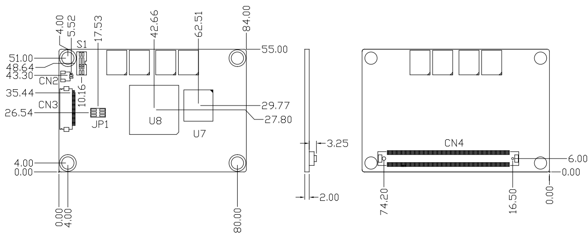
Component Side
