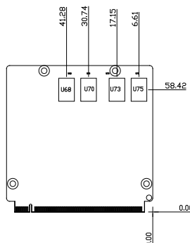
Solder Side
