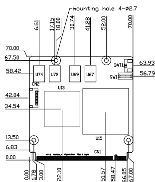
Component Side
