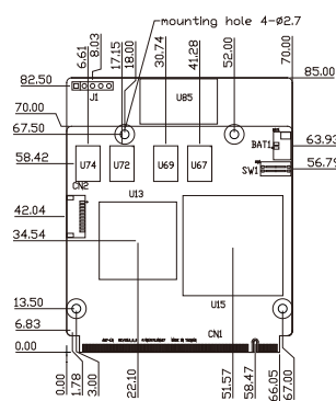
Component Side
