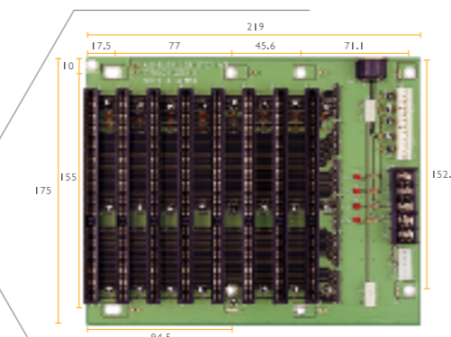
BP-208SI-A00 > Segments : 1 Segments > Slot : 8 x ISA
