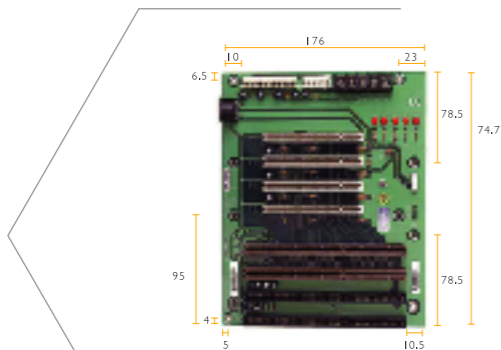
BP-208SS-P4-V10 > Segments : 1 Segment > Slot : 2 x PCISA , 4 X PCI , 2 x ISA
