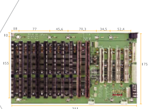
BP-214SS-P4-V11 > Segments : 1 Segment > Slot : 2 x PCISA , 4 X PCI , 8 x ISA > Chassis : ARC-6414
