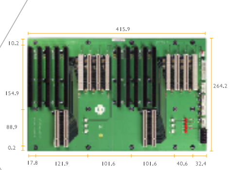
BP-218DG-P8-V61 > Segments : 2 Segment > Slot : 4 x PICMG , 8 X PCI , 6 x ISA > Chassis : ARC-6620
