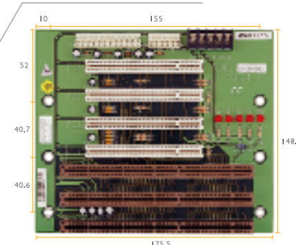
BP-206SS-P4-A12 > Segments : 1 Segment > Slot : 3 x PCISA , 4 x PCI
