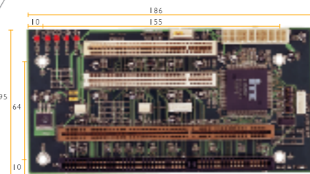
BP-204SS-P2-A10 > Segments : 1 Segment > Slot : 1 x PICMG , 1 x PCI , 1 x ISA 1 x PCISA , 1 x PCI , 1 x ISA > Chassis : AEC-204
