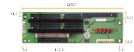
BP-206SG-P2-VII ( Dual-side ) > Segments : 1 Segment > Slot : 1 x PICMG , 2 X PCI , 3 x ISA > Chassis : ARC-6205
