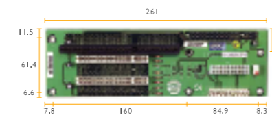
BP-206SG-P4-V00 ( Dual-side ) > Segments : 1 Segment > Slot : 1 x PICMG , 4 x PCI , 1 x ISA > Chassis : ARC-6205
